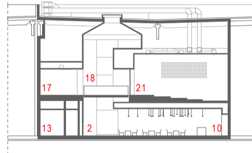
B-B section scale 1:400
