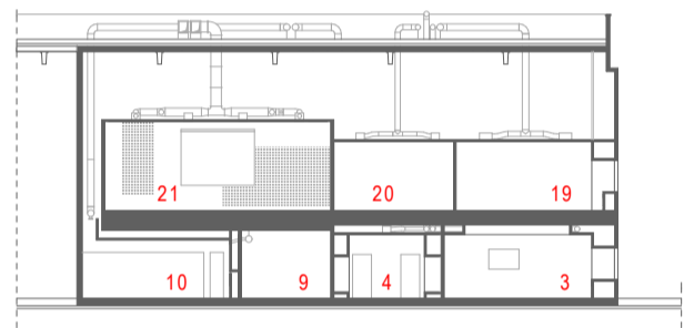
C-C section scale 1:400
