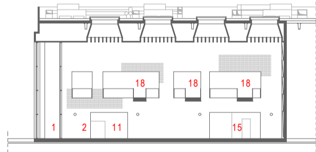
E-E section scale 1:400
