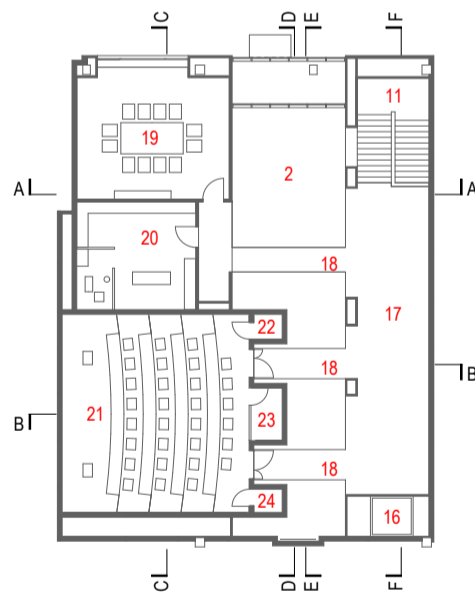
upper floor scale 1:400
