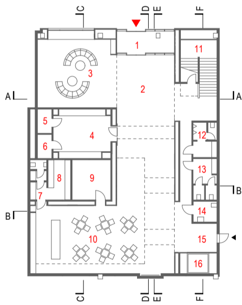
ground floor scale 1:400
