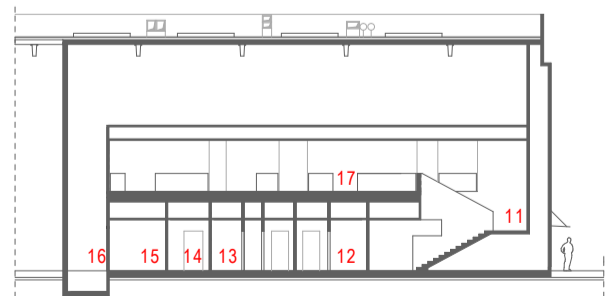
F-F section scale 1:400
